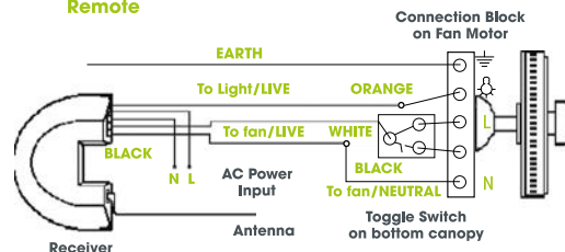
Forward/reverse toggle switch
