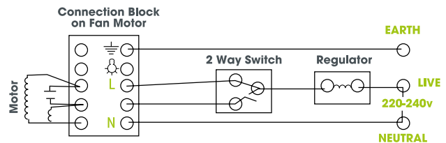
5 Speed Regulator & 1 x 2 way Light Switch
